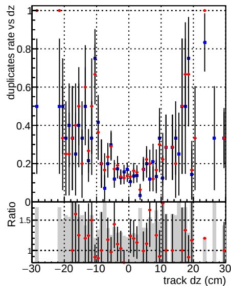
al mkFit10muon-base1 RECO al mkFit10muon-base2 RECO
