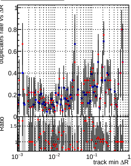
Legend: DQM_V0001_R000000001_Global_mkFit10muon-base1_RECO (blue squares), DQM_V0001_R000000001_Global_mkFit10muon-base2_RECO (red circles)
