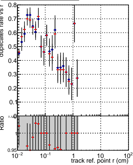
■ DQM_V0001_R000000001_Global_mkFit10muon-base1_RECO ● DQM_V0001_R000000001_Global_mkFit10muon-base2_RECO
