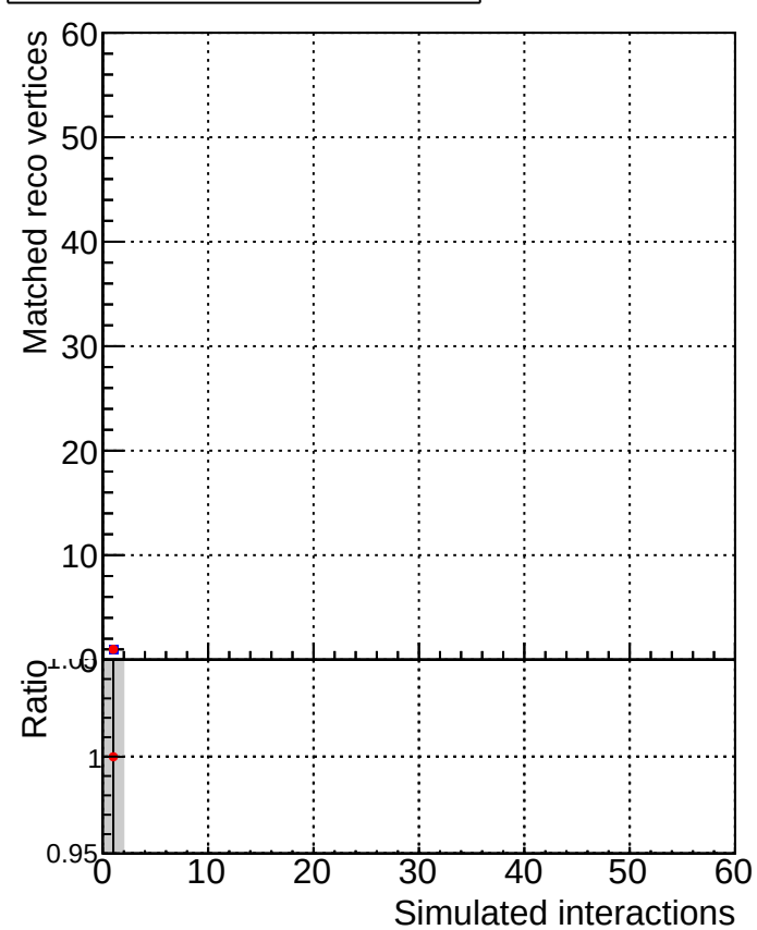
MatchedRecoVtx_vs_GenVtx
