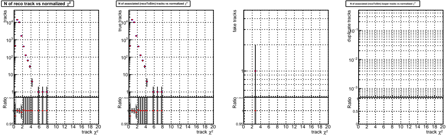
N of reco track vs. \chi^2 DQM_V0001_R0000000001_Global_mkFit10muon-base1_RECO DQM_V0001_R0000000001_Global_mkFit10muon-base2_RECO
