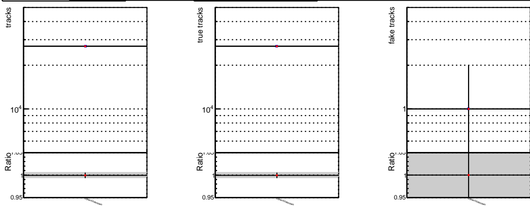
N of reco track vs. \chi^2 DQM_V0001_R0000000001_Global_mkFit10muon-base1_RECO DQM_V0001_R0000000001_Global_mkFit10muon-base2_RECO
