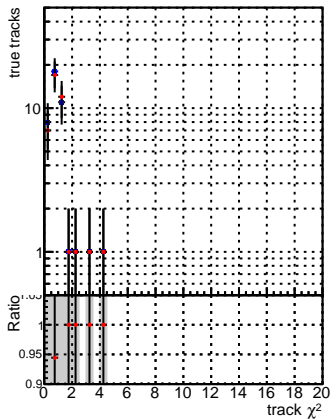
N of reco track vs. \chi^2 DQM_V0001_R000000001 Global_mkFit10muon-base1_RECO DQM_V0001_R000000001 Global_mkFit10muon-base2_RECO
