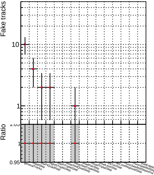
Number —●— DQM_V0001 R000000001 Global mkFit10muon-base2 RECO
