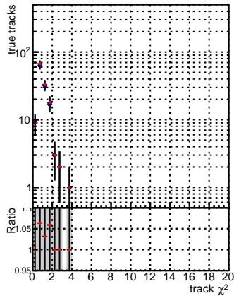
Legend for the plots: Global_mkFit10muon-base1_RECO Global_mkFit10muon-base2_RECO DQM_V0001_R000000001 DQM_V0001_R000000001
