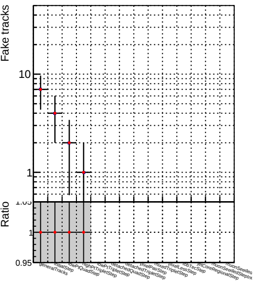
Number ● DQM_V0001_R000000001_Global_mkFit10muon-base2_RECO
