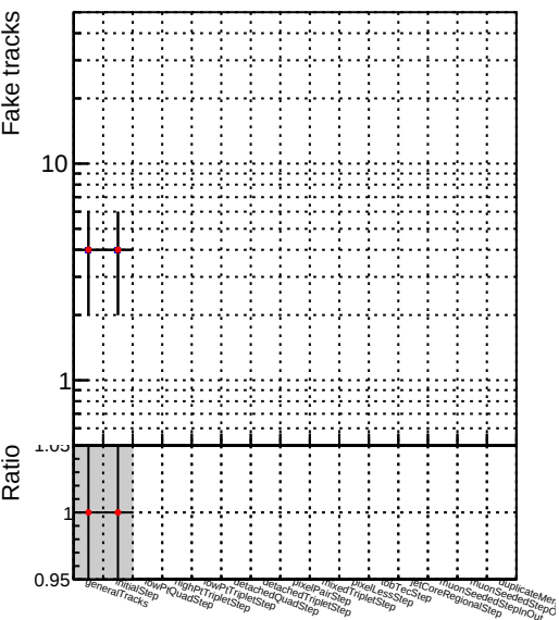
Number ● DQM_V0001_R000000001_Global_mkFit10muon-base2_RECO
