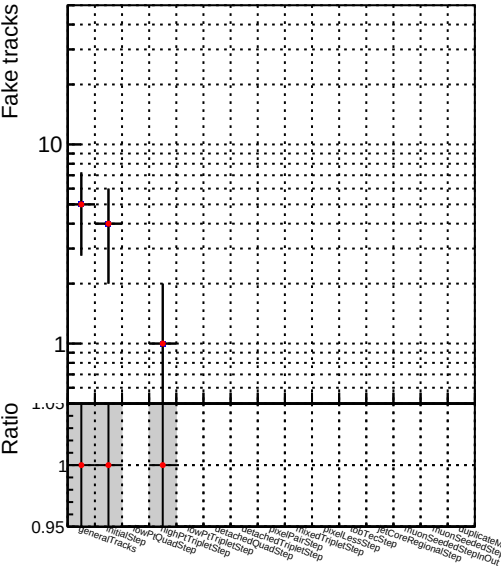
Number ● DQM_V0001_R000000001_Global_mkFit10muon-base2_RECO
