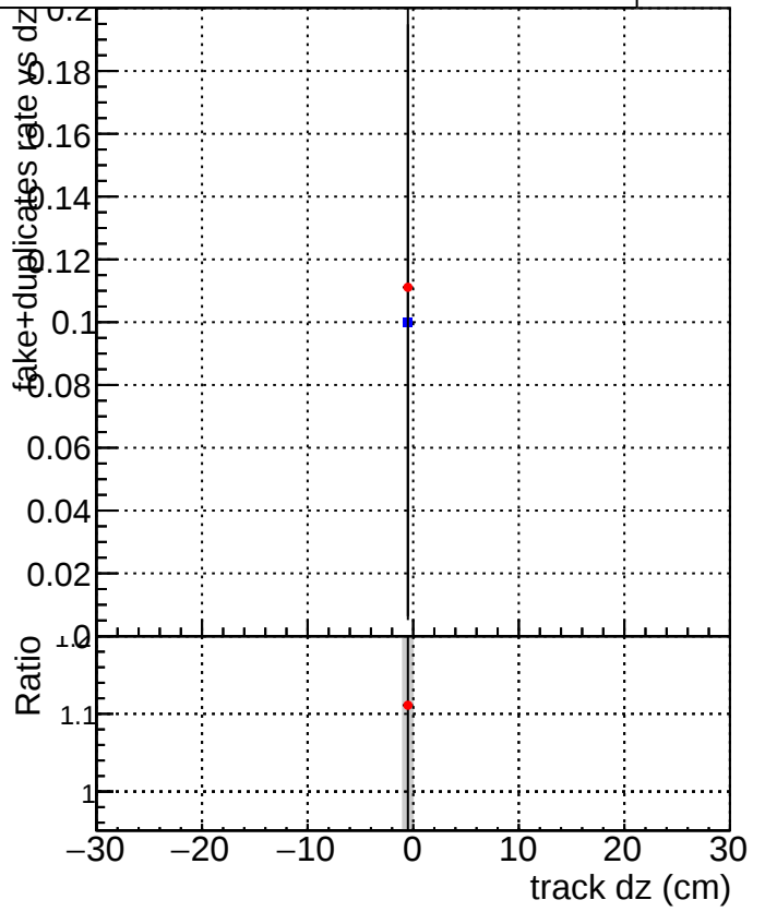
DQM_V0001_R000000001_Global_mkFit10muon-base1_RECO DQM_V0001_R000000001_Global_mkFit10muon-base2_RECO
