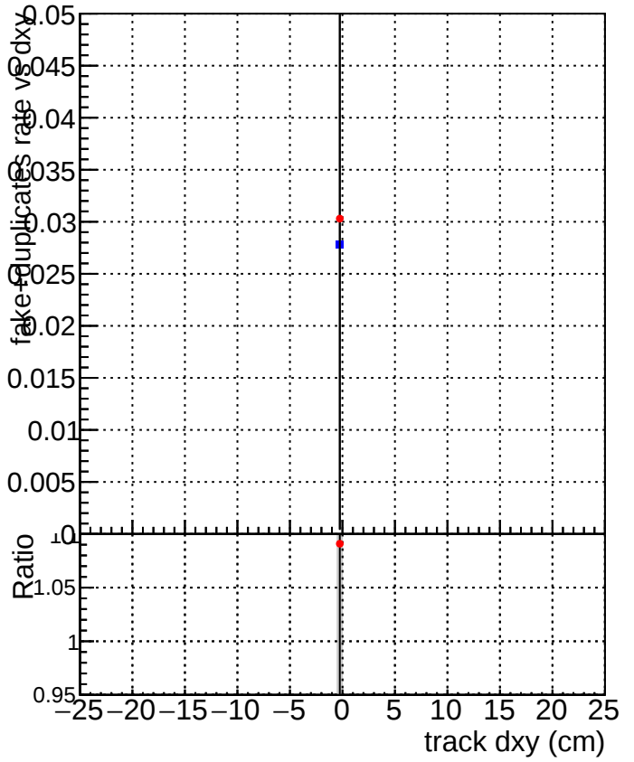
DQM_V0001_R000000001_Global_mkFit10muon-base1_RECO DQM_V0001_R000000001_Global_mkFit10muon-base2_RECO
