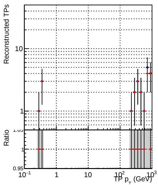
—•— DQM_V0001_R0000000001_Global_mkFit10muon-base1_RECO —•— DQM_V0001_R0000000001_Global_mkFit10muon-base2_RECO
