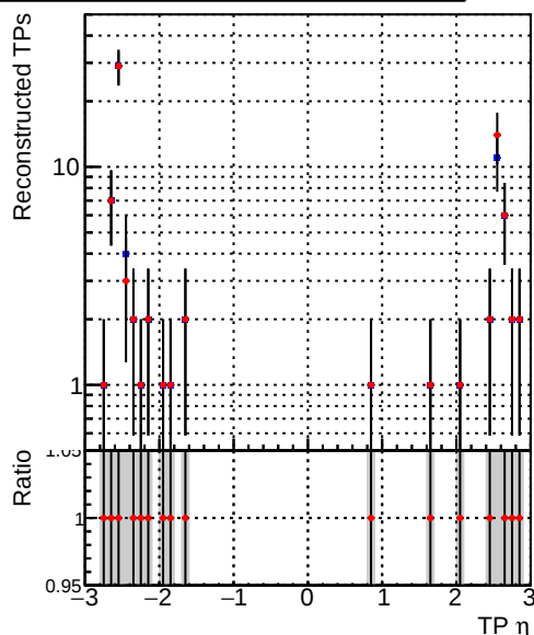
—•— DQM_V0001_R0000000001_Global_mkFit10muon-base1_RECO —•— DQM_V0001_R0000000001_Global_mkFit10muon-base2_RECO
