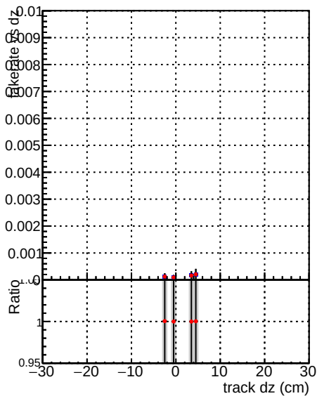
█ DQM_V0001_R0000000001 Global mkFit10muon-base1 RECO █ DQM_V0001_R0000000001 Global mkFit10muon-base2 RECO
