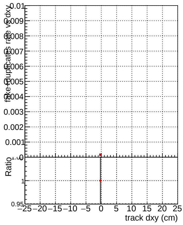
DQM_V0001_R000000001_Global_mkFit10muon-base1_RECO
