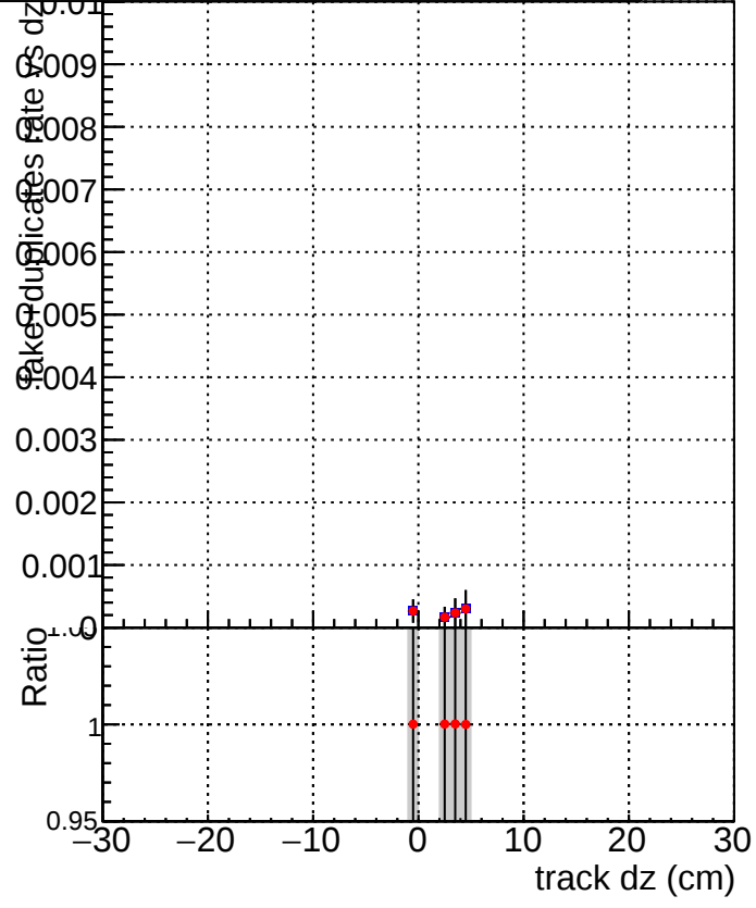
DQM_V0001_R000000001_Global_mkFit10muon-base1_RECO
