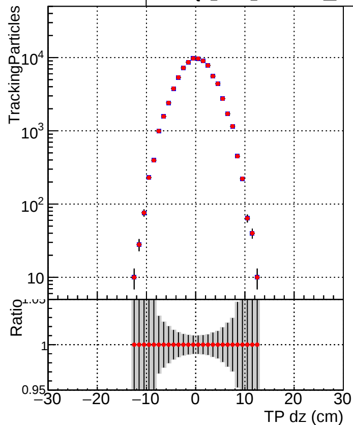
N of simulated track Legend: DQM_V0001_R000000001_Global_mkFit10muon-base1_RECO DQM_V0001_R000000001_Global_mkFit10muon-base2_RECO
