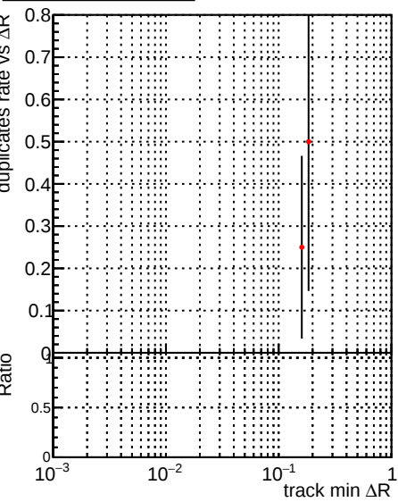
Legend: - Blue line with error bars: DQM_V0001_R000000001_Global_mkFit10muon-base1_RECO - Red line with error bars: DQM_V0001_R000000001_Global_mkFit10muon-base2_RECO
