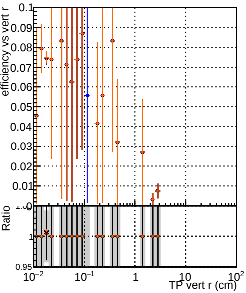
Efficiency vs vertpos —•— DQM_noFit2_step2_ttbar-phase1-newgeom —•— DQM_Fit2_step2_ttbar-phase1-newgeom —•— DQM_Fit2AndCPEGeneric_step2_ttbar-phase1-newgeom —•— DQM_Fit2AndCPETemplate_step2_ttbar-phase1-newgeom
