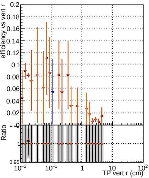
Efficiency vs TP vert r (cm) —•— DQM_noFit2_step2_ttbar-phase1-newgeom —•— DQM_Fit2_step2_ttbar-phase1-newgeom —•— DQM_Fit2AndCPEGeneric_step2_ttbar-phase1-newgeom —•— DQM_Fit2AndCPETemplate_step2_ttbar-phase1-newgeom
