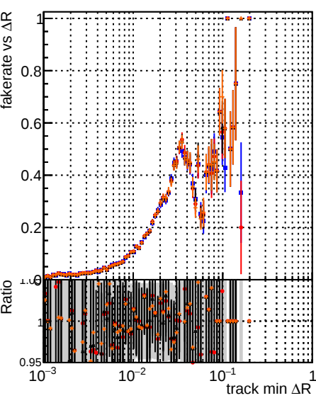
Fake rate vs \Delta R (track, jet) DOM noFit2 step2 ttbar-phase1-newgeom DOM noFit2 step2 ttbar-phase1-newgeom DOM noFit2 step2 ttbar-phase1-newgeom DOM noFit2 step2 ttbar-phase1-newgeom
