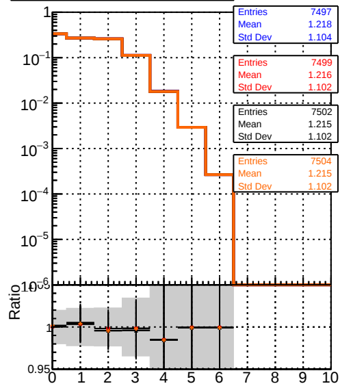
— DQM_noFit2_step2_ttbar-phase1-newgeom — DQM_Fit2_step2_ttbar-phase1-newgeom — DQM_Fit2AndCPEGeneric_step2_ttbar-phase1-newgeom — DQM_Fit2AndCPETemplate_step2_ttbar-phase1-newgeom
