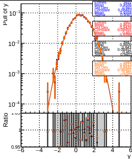
RecoPVAssoc2GenPVMatched_PullY Legend: DOM no Fit2_step2_ttbare-phase1-newgeom DOM Fit2_step2_ttbare-phase1-newgeom DOM Fit2_and_PEGeneric_step2_ttbare-phase1-newgeom DOM Fit2_and_PEGeneric_step2_ttbare-phase1-newgeom
