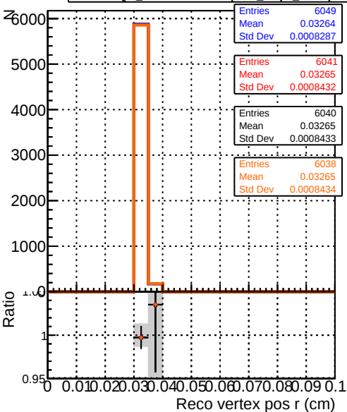
Recons Legend: Blue line: DQM_noFit2_step2_ttbar-phase1-newgeom Red line: DQM_Fit2_step2_ttbar-phase1-newgeom Black line: DQM_Fit2AndCPEGeneric_step2_ttbar-phase1-newgeom Orange line: DQM_Fit2AndCPETemplate_step2_ttbar-phase1-newgeom
