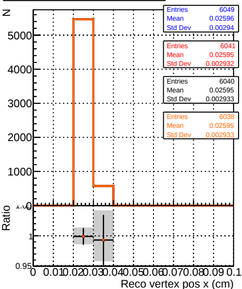
Recons Legend: Blue line: DQM_noFit2_step2_ttbar-phase1-newgeom Red line: DQM_Fit2_step2_ttbar-phase1-newgeom Black line: DQM_Fit2AndCPEGeneric_step2_ttbar-phase1-newgeom Orange line: DQM_Fit2AndCPETemplate_step2_ttbar-phase1-newgeom
