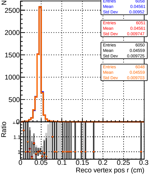
Recons Legend: - DQM_noFit2_step2_ttbar-phase1-newgeom (blue line) - DQM_Fit2_step2_ttbar-phase1-newgeom (red line) - DQM_Fit2AndCPEGeneric_step2_ttbar-phase1-newgeom (black line) - DQM_Fit2AndCPETemplate_step2_ttbar-phase1-newgeom (orange line)
