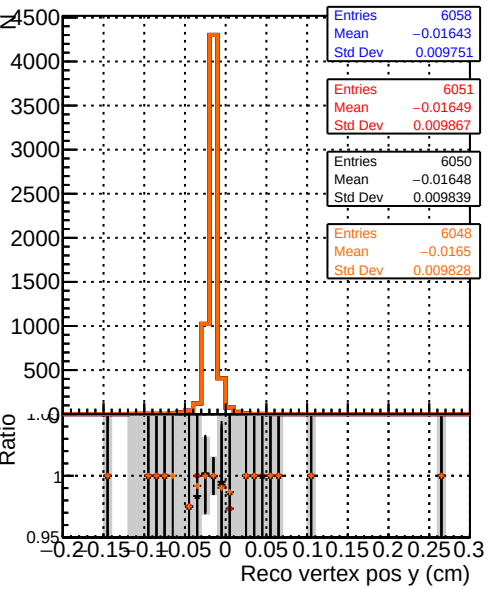
Recons Legend: - DQM_noFit2_step2_ttbar-phase1-newgeom (blue line) - DQM_Fit2_step2_ttbar-phase1-newgeom (red line) - DQM_Fit2AndCPEGeneric_step2_ttbar-phase1-newgeom (black line) - DQM_Fit2AndCPETemplate_step2_ttbar-phase1-newgeom (orange line)
