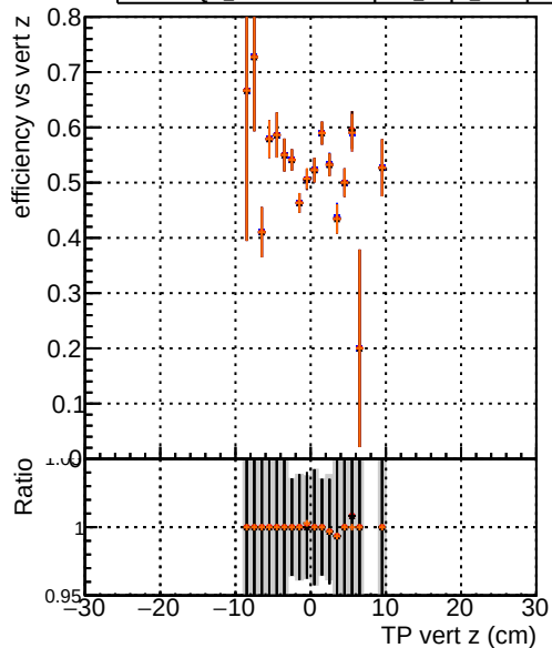
Efficiency vs vert z —•— DQM_noFit2_step2_ttbar-phase1-newgeom —•— DQM_Fit2_step2_ttbar-phase1-newgeom —•— DQM_Fit2AndCPEGeneric_step2_ttbar-phase1-newgeom —•— DQM_Fit2AndCPETemplate_step2_ttbar-phase1-newgeom
