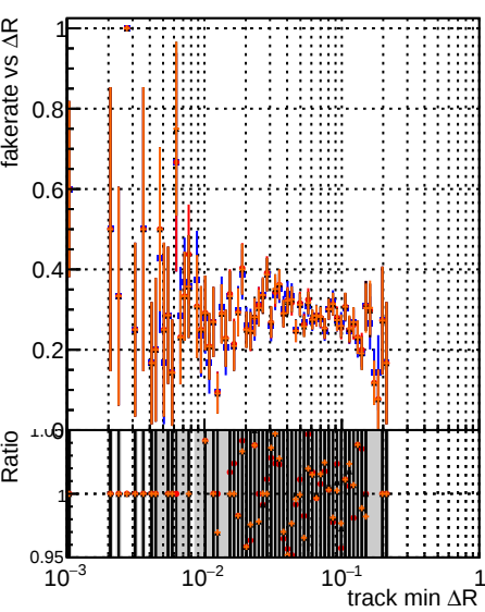
Fake rate vs \Delta R (track, jet) DOM noFit2_step2_ttbbar-phase1-newgeom DOM Fit2_step2_ttbbar-phase1-newgeom DOM Fit2AndCPETemplate_step2_ttbbar-phase1-newgeom
