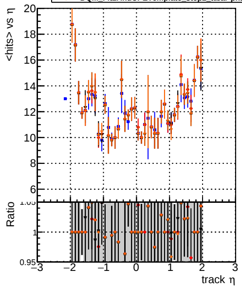
— DQM_noFit2_step2_ttbar-phase1-newgeom — DQM_Fit2_step2_ttbar-phase1-newgeom — DQM_Fit2AndCPEGeneric_step2_ttbar-phase1-newgeom — DQM_Fit2AndCPETemplate_step2_ttbar-phase1-newgeom mean hit
