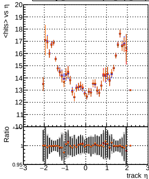
mean hit — DQM_noFit2_step2_ttbar-phase1-newgeom — DQM_Fit2_step2_ttbar-phase1-newgeom — DQM_Fit2AndCPEGeneric_step2_ttbar-phase1-newgeom — DQM_Fit2AndCPETemplate_step2_ttbar-phase1-newgeom
