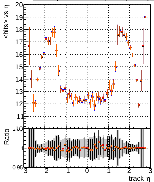
mean hits vs \eta DQM_noFit2_step2_ttbbar-phase1-newgeom DQM_Fit2_step2_ttbbar-phase1-newgeom DQM_Fit2AndCPEGeneric_step2_ttbbar-phase1-newgeom DQM_Fit2AndCPETemplate_step2_ttbbar-phase1-newgeom
