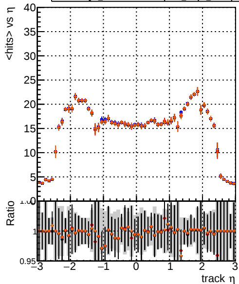
mean hits vs \eta — DQM_noFit2_step2_ttbbar-phase1-newgeom — DQM_Fit2_step2_ttbbar-phase1-newgeom — DQM_Fit2AndCPEGeneric_step2_ttbbar-phase1-newgeom — DQM_Fit2AndCPETemplate_step2_ttbbar-phase1-newgeom
