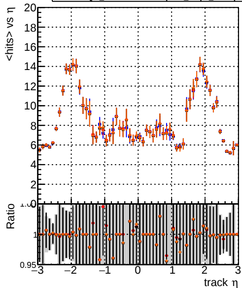
— DQM_noFit2_step2_ttbar-phase1-newgeom — DQM_Fit2_step2_ttbar-phase1-newgeom — DQM_Fit2AndCPEGeneric_step2_ttbar-phase1-newgeom — DQM_Fit2AndCPETemplate_step2_ttbar-phase1-newgeom mean hits
