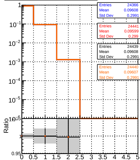
— DQM_noFit2_step2_ttbbar-phase1-newgeom — DQM_Fit2_step2_ttbbar-phase1-newgeom — DQM_Fit2AndCPEGeneric_step2_ttbbar-phase1-newgeom — DQM_Fit2AndCPETemplate_step2_ttbbar-phase1-newgeom
