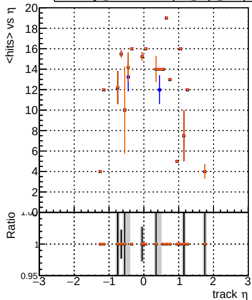
Legend: Blue line: DQM_noFit2_step2_ttbar-phase1-newgeom Red line: DQM_Fit2_step2_ttbar-phase1-newgeom Black line: DQM_Fit2AndCPEGeneric_step2_ttbar-phase1-newgeom Orange line: DQM_Fit2AndCPETemplate_step2_ttbar-phase1-newgeom mean hits
