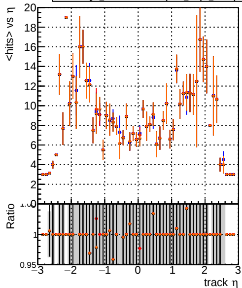
Legend: — DQM_noFit2_step2_ttbar-phase1-newgeom — DQM_Fit2_step2_ttbar-phase1-newgeom — DQM_Fit2AndCPEGeneric_step2_ttbar-phase1-newgeom — DQM_Fit2AndCPETemplate_step2_ttbar-phase1-newgeom
