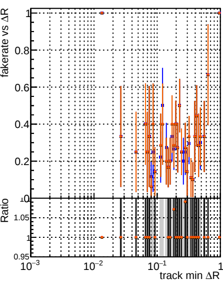
Fake rate vs \Delta R(\text{track, jet}) Legend: DOM (blue) noFit2 (red) step2 (black) ttbar-phase1-newgeom (orange)
