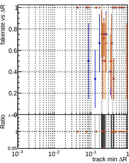
Fake rate vs \Delta R(\text{track, jet}) Legend: DOM noFit2_step2_ttbar-phase1-newgeom DOM noFit2_step2_ttbar-phase1-newgeom DOM noFit2_step2_ttbar-phase1-newgeom DOM noFit2_step2_ttbar-phase1-newgeom
