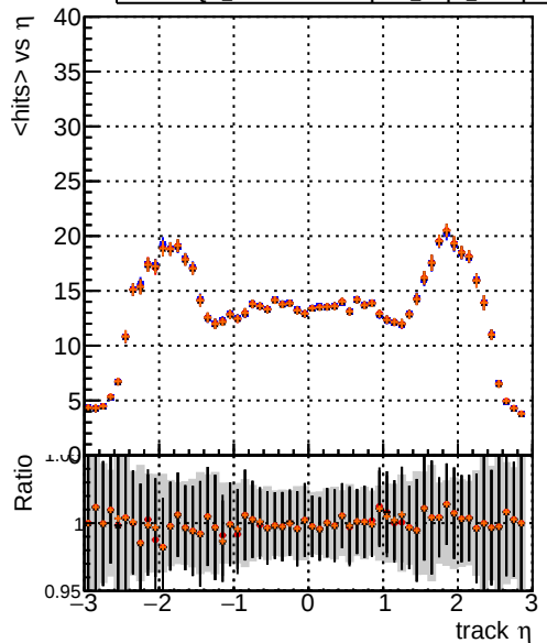
mean hits DQM_noFit2_step2_ttbar-phase1-newgeom DQM_Fit2_step2_ttbar-phase1-newgeom DQM_Fit2AndCPEGeneric_step2_ttbar-phase1-newgeom DQM_Fit2AndCPETemplate_step2_ttbar-phase1-newgeom
