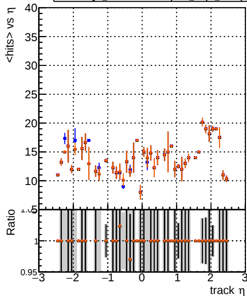
— DQM_noFit2_step2_ttbar-phase1-newgeom — DQM_Fit2_step2_ttbar-phase1-newgeom — DQM_Fit2AndCPETemplate_step2_ttbar-phase1-newgeom — DQM_Fit2AndCPETemplate_step2_ttbar-phase1-newgeom mean hit
