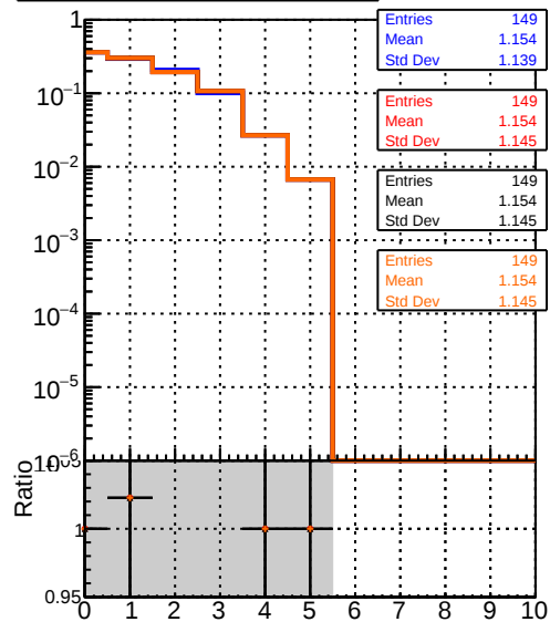
— DQM_noFit2_step2_ttbar-phase1-newgeom — DQM_Fit2_step2_ttbar-phase1-newgeom — DQM_Fit2AndCPETemplate_step2_ttbar-phase1-newgeom — DQM_Fit2AndCPETemplate_step2_ttbar-phase1-newgeom mean hit
