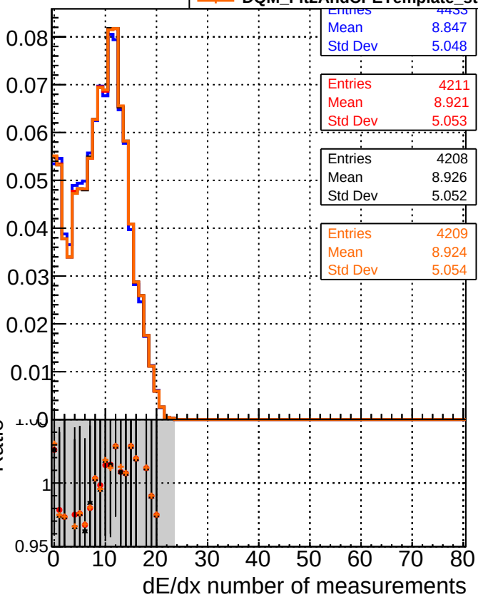
— DQM_noFit2_step2_ttbar-phase1-newgeom — DQM_Fit2_step2_ttbar-phase1-newgeom — DQM_Fit2AndCPEGeneric_step2_ttbar-phase1-newgeom — DQM_Fit2AndCPETemplate_step2_ttbar-phase1-newgeom
