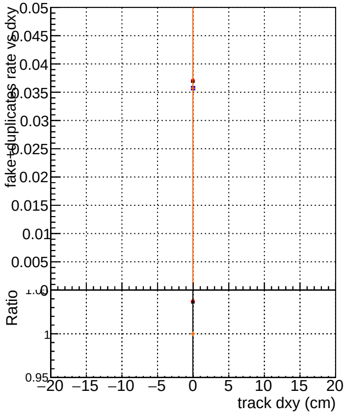
DQM_noFit2_step2_ttbar-phase1-newgeom DQM_Fit2_step2_ttbar-phase1-newgeom DQM_Fit2AndCPEGeneric_step2_ttbar-phase1-newgeom DQM_Fit2AndCPETemplate_step2_ttbar-phase1-newgeom
