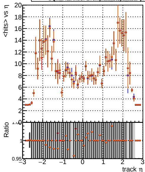
mean hit — DQM_noFit2_step2_ttbar-phase1-newgeom — DQM_Fit2_step2_ttbar-phase1-newgeom — DQM_Fit2AndCPEGeneric_step2_ttbar-phase1-newgeom — DQM_Fit2AndCPETemplate_step2_ttbar-phase1-newgeom
