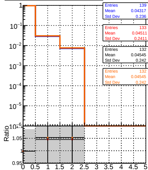
mean hit DQM_noFit2_step2_ttbar-phase1-newgeom DQM_Fit2_step2_ttbar-phase1-newgeom DQM_Fit2AndCPEGeneric_step2_ttbar-phase1-newgeom DQM_Fit2AndCPETemplate_step2_ttbar-phase1-newgeom
