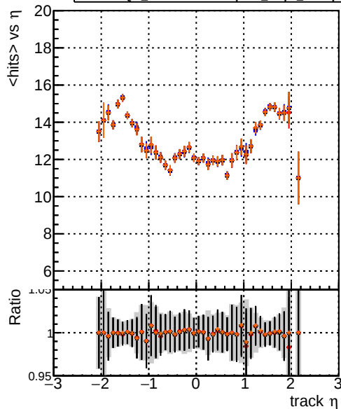
mean hits vs \eta — DQM_noFit2_step2_ttbar-phase1-newgeom — DQM_Fit2_step2_ttbar-phase1-newgeom — DQM_Fit2AndCPEGeneric_step2_ttbar-phase1-newgeom — DQM_Fit2AndCPETemplate_step2_ttbar-phase1-newgeom
