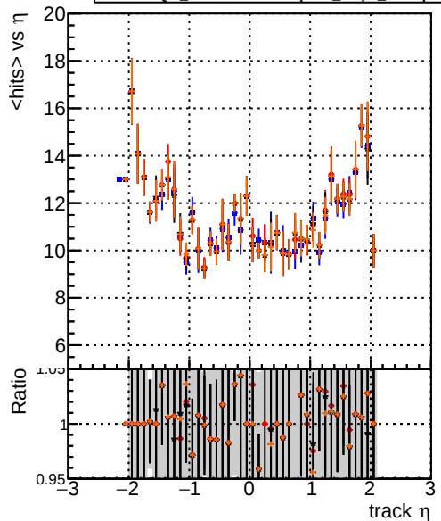
— DQM_noFit2_step2_ttbbar-phase1-newgeom — DQM_Fit2_step2_ttbbar-phase1-newgeom — DQM_Fit2AndCPEGeneric_step2_ttbbar-phase1-newgeom — DQM_Fit2AndCPETemplate_step2_ttbbar-phase1-newgeom mean hit
