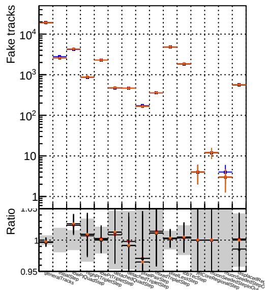
Number Legend 1 DQM_noFit2_step2_ttbar-phase1-newgeom 2 DQM_Fit2_step2_ttbar-phase1-newgeom 3 DQM_Fit2AndCPEGeneric_step2_ttbar-phase1-newgeom 4 DQM_Fit2AndCPETemplate_step2_ttbar-phase1-newgeom
