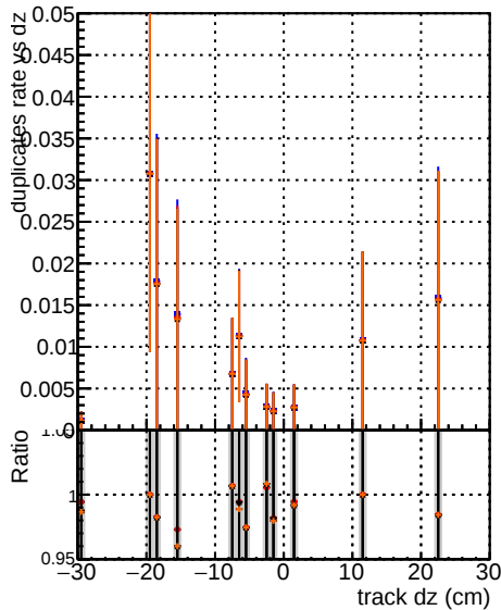
2 ttbar-phase1-newgeom p2 ttbar-phase1-newgeom
