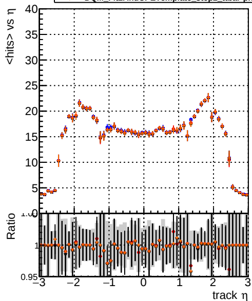
mean hits vs \eta — DQM_noFit2_step2_ttbbar-phase1-newgeom — DQM_Fit2_step2_ttbbar-phase1-newgeom — DQM_Fit2AndCPEGeneric_step2_ttbbar-phase1-newgeom — DQM_Fit2AndCPETemplate_step2_ttbbar-phase1-newgeom
