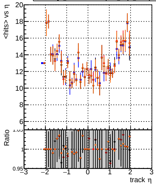
Legend: — DQM_noFit2_step2_ttbar-phase1-newgeom — DQM_Fit2_step2_ttbar-phase1-newgeom — DQM_Fit2AndCPEGeneric_step2_ttbar-phase1-newgeom — DQM_Fit2AndCPETemplate_step2_ttbar-phase1-newgeom
