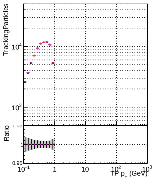
—•— DOM original_step2_ttbar-phase1-newgeom —•— DOM mkFit_step2_ttbar-phase1-newgeom —•— DOM angle_step2_ttbar-phase1-newgeom —•— DOM fast_step2_ttbar-phase1-newgeom —•— DOM pixelCPEtemplate_step2_ttbar-phase1-newgeom
