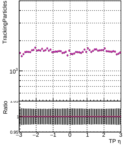
— DOM original_step2_ttbar-phase1-newgeom — DOM mkFit_step2_ttbar-phase1-newgeom — DOM angle_step2_ttbar-phase1-newgeom — DOM fast_step2_ttbar-phase1-newgeom — DOM pixelCPEtemplate_step2_ttbar-phase1-newgeom
